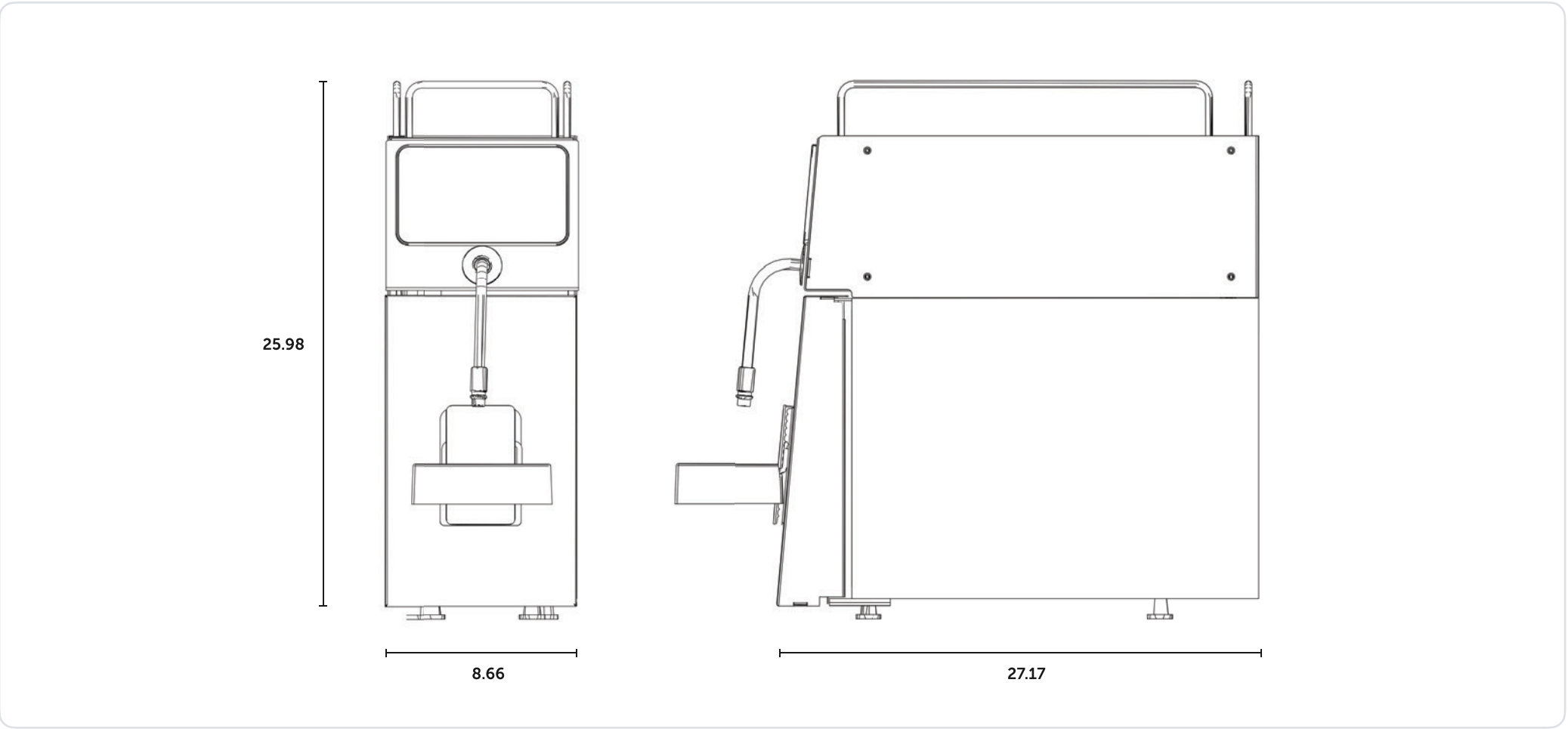
Dimensions (WxHxD): 8.66 in x 25.98 in x 27.17 in
